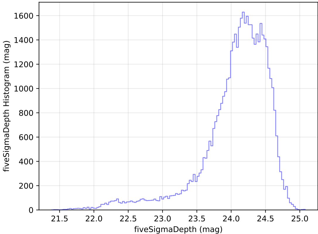
too_elab_r32_d2_griz_v3.4_10yrs Yr 1 r band: fiveSigmaDepth Histogram
