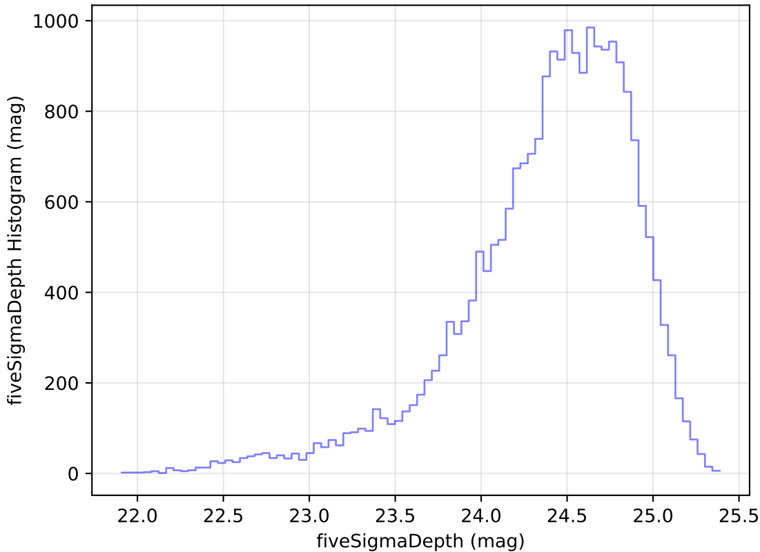
too_elab_r32_d2_griz_v3.4_10yrs Yr 1 g band: fiveSigmaDepth Histogram
