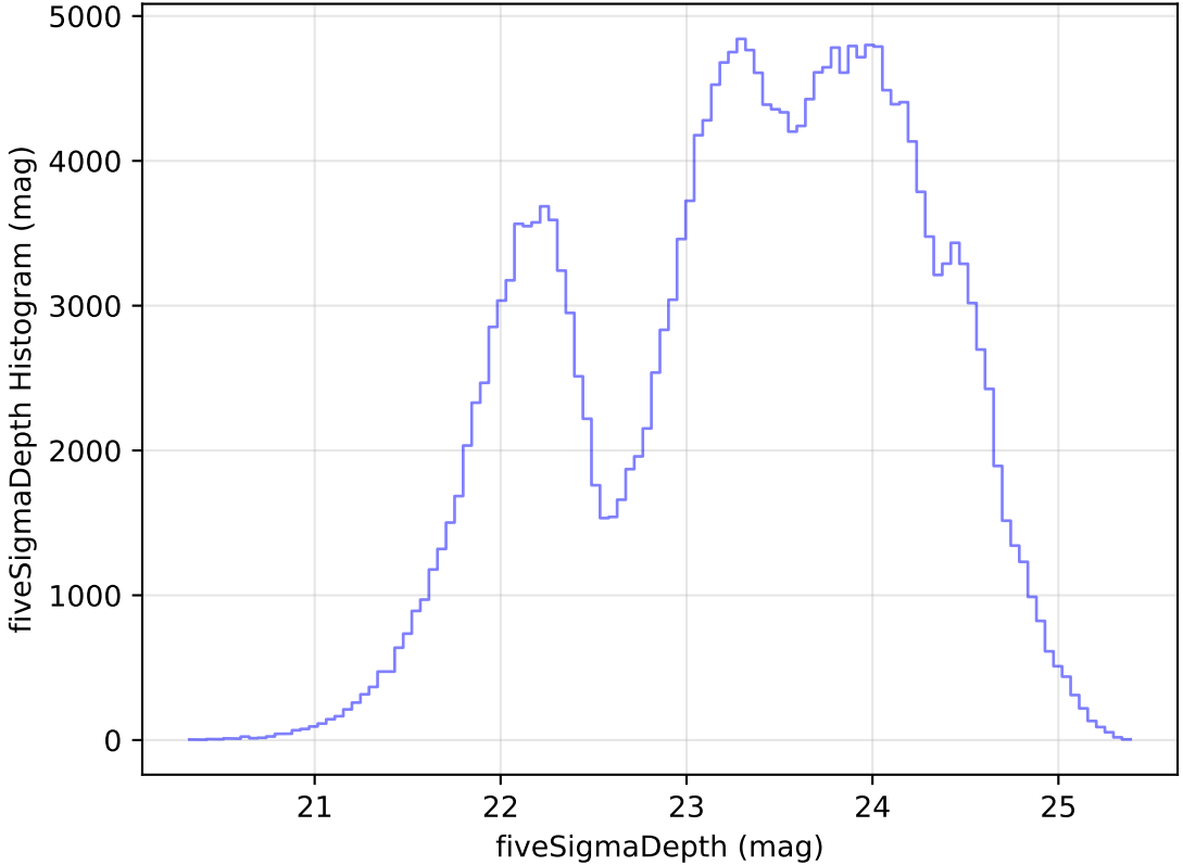
too_elab_r32_d2_griz_v3.4_10yrs Yr 1 all bands: fiveSigmaDepth Histogram
