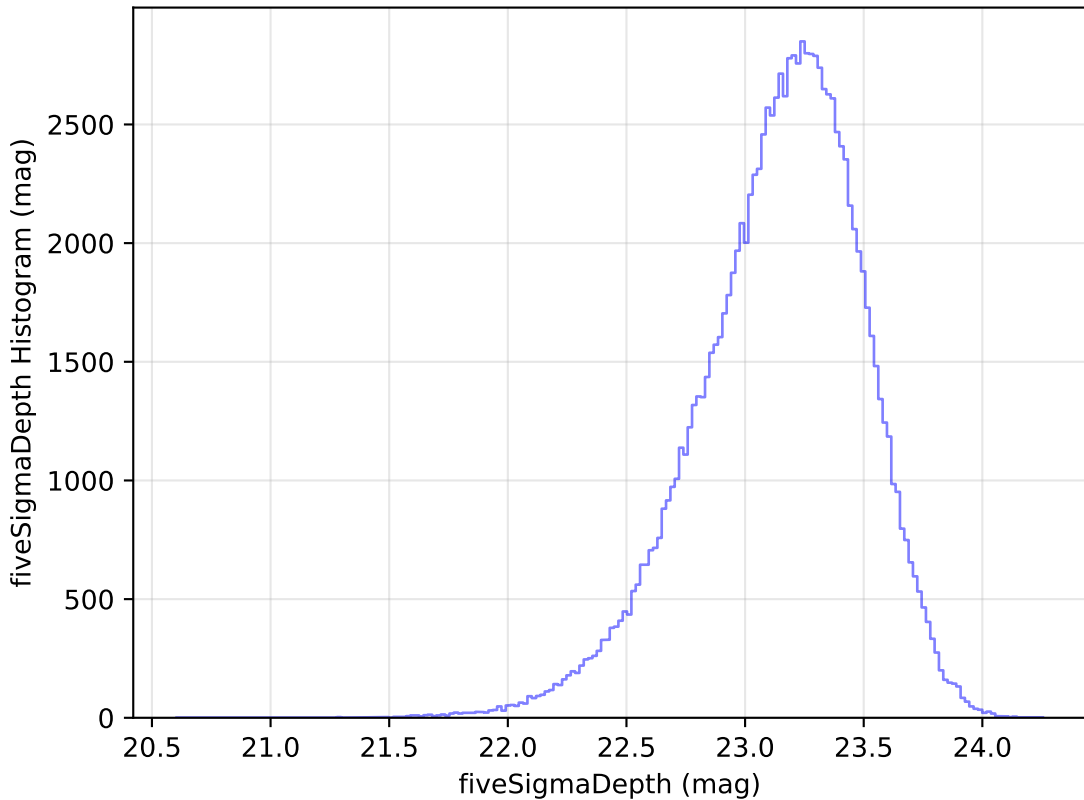
too_elab_r32_d2_griz_v3.4_10yrs WFD u band: fiveSigmaDepth Histogram
