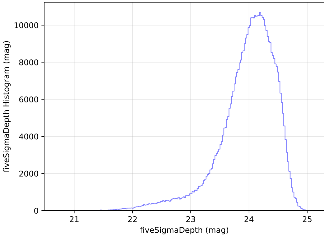
too_elab_r32_d2_griz_v3.4_10yrs WFD r band: fiveSigmaDepth Histogram
