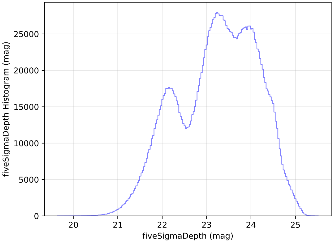
too_elab_r32_d2_griz_v3.4_10yrs WFD all bands: fiveSigmaDepth Histogram
