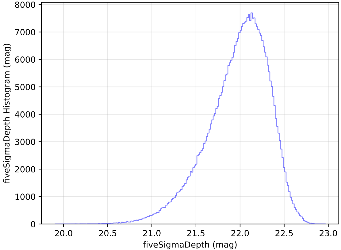
too_elab_r32_d2_griz_v3.4_10yrs All sky y band: fiveSigmaDepth Histogram
