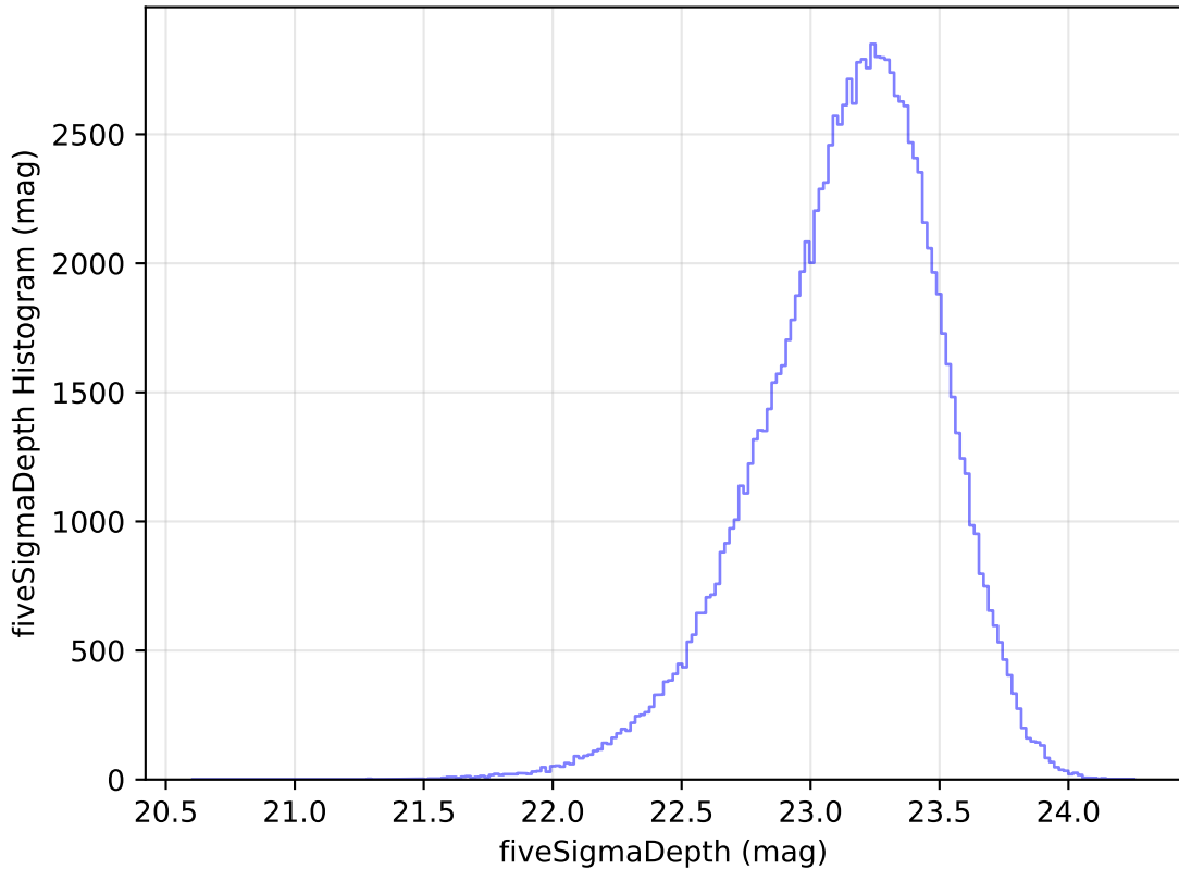
too_elab_r32_d2_griz_v3.4_10yrs All sky u band: fiveSigmaDepth Histogram
