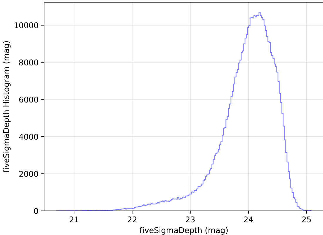
too_elab_r32_d2_griz_v3.4_10yrs All sky r band: fiveSigmaDepth Histogram
