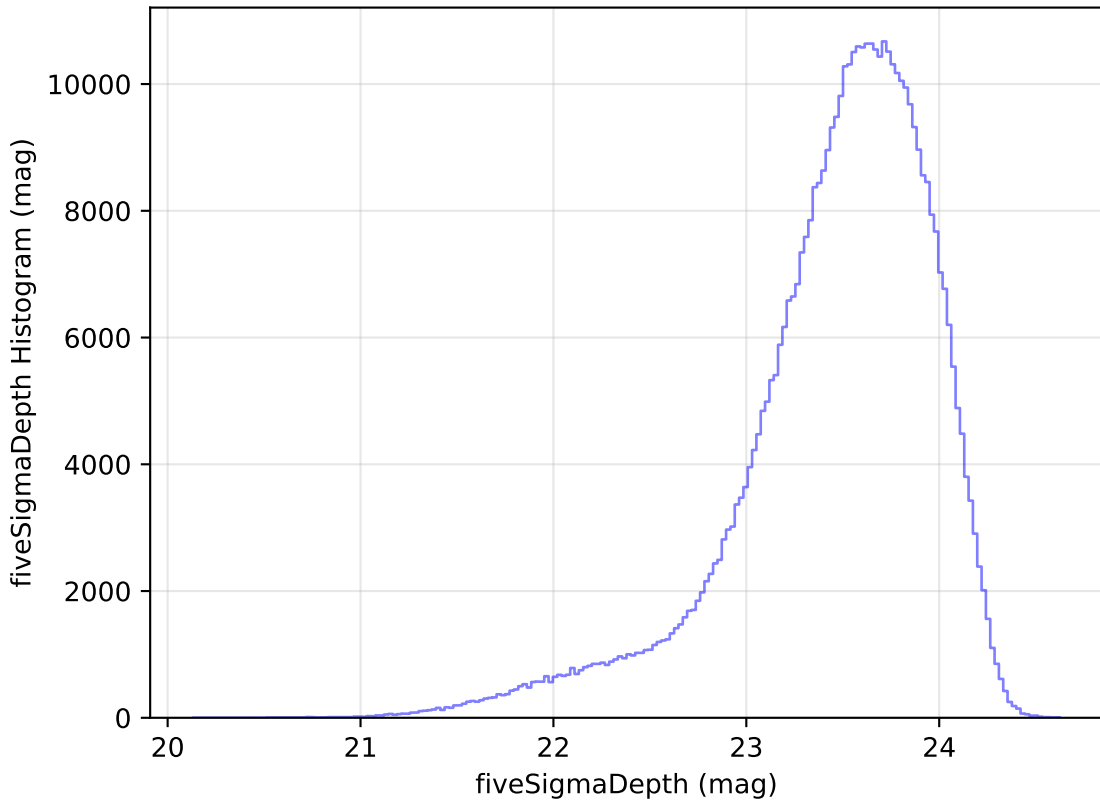
too_elab_r32_d2_griz_v3.4_10yrs All sky i band: fiveSigmaDepth Histogram
