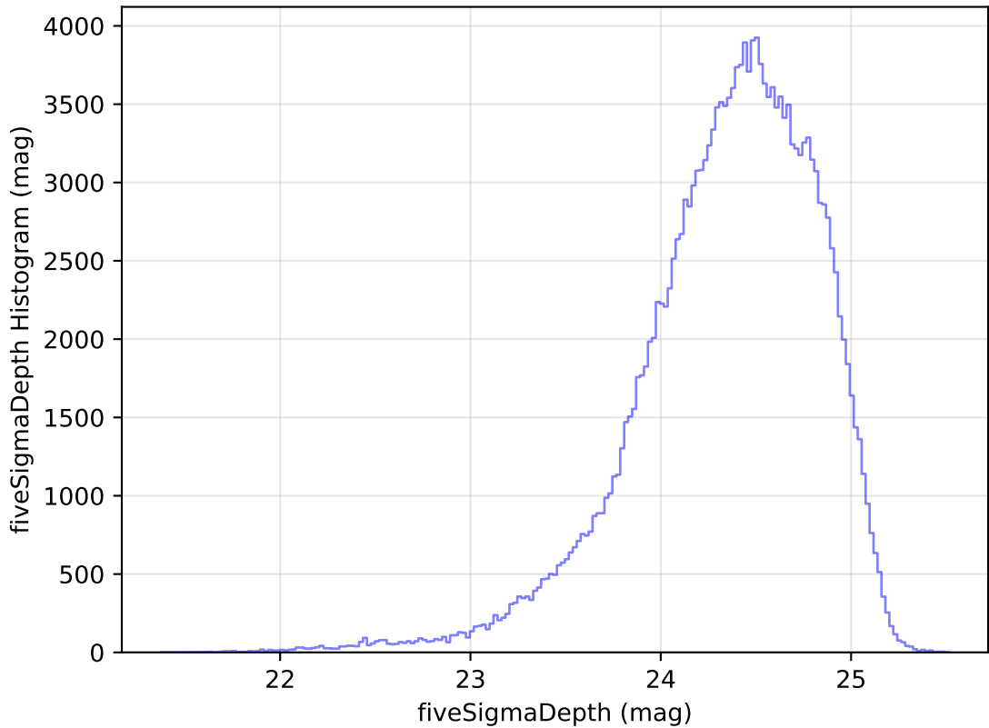
too_elab_r32_d2_griz_v3.4_10yrs All sky g band: fiveSigmaDepth Histogram
