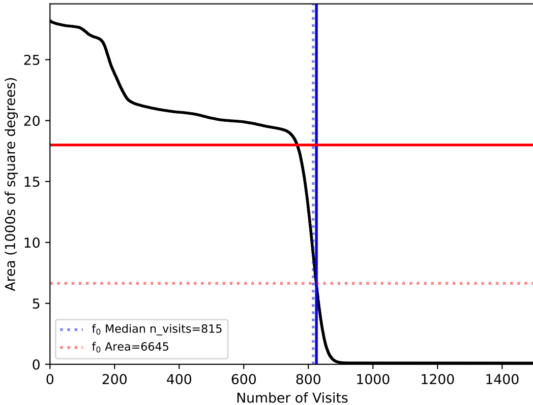
too_elab_r32_d2_griz_v3.4_10yrs All sky: fO
