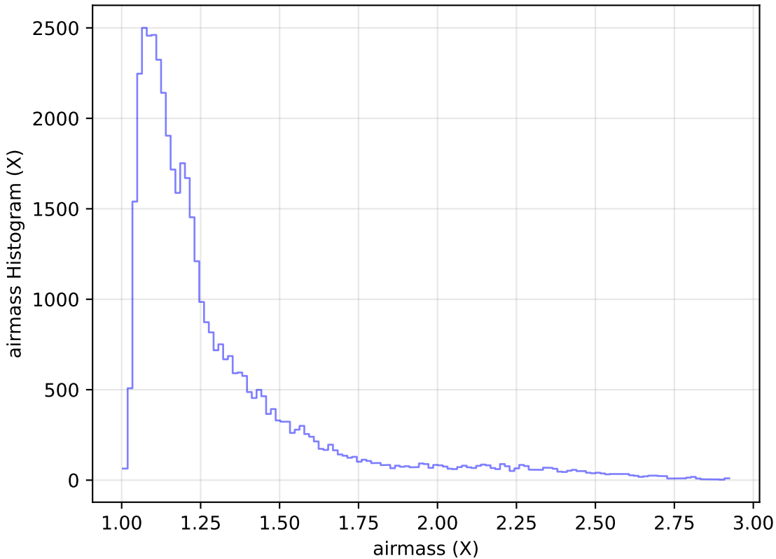
too_elab_r32_d2_griz_v3.4_10yrs Yr 1 z band: airmass Histogram
