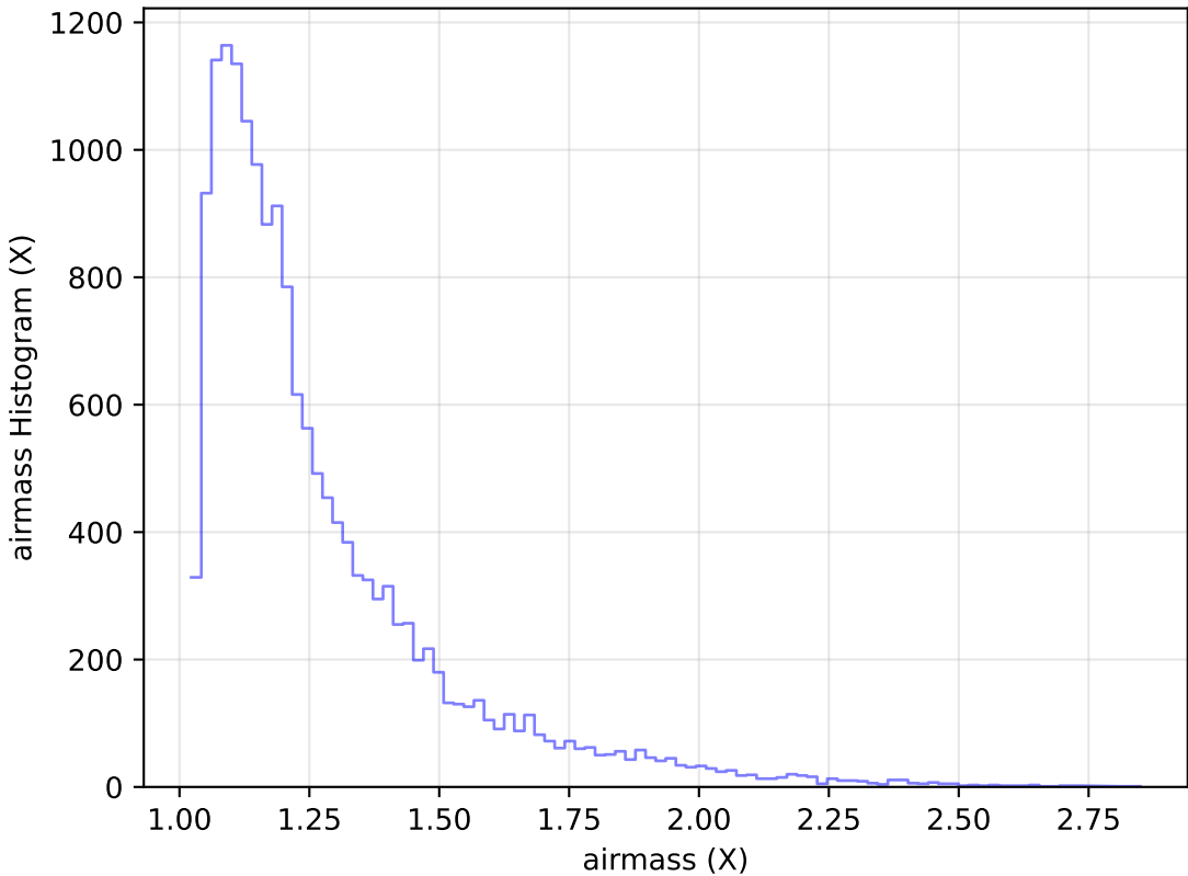
too_elab_r32_d2_griz_v3.4_10yrs Yr 1 u band: airmass Histogram
