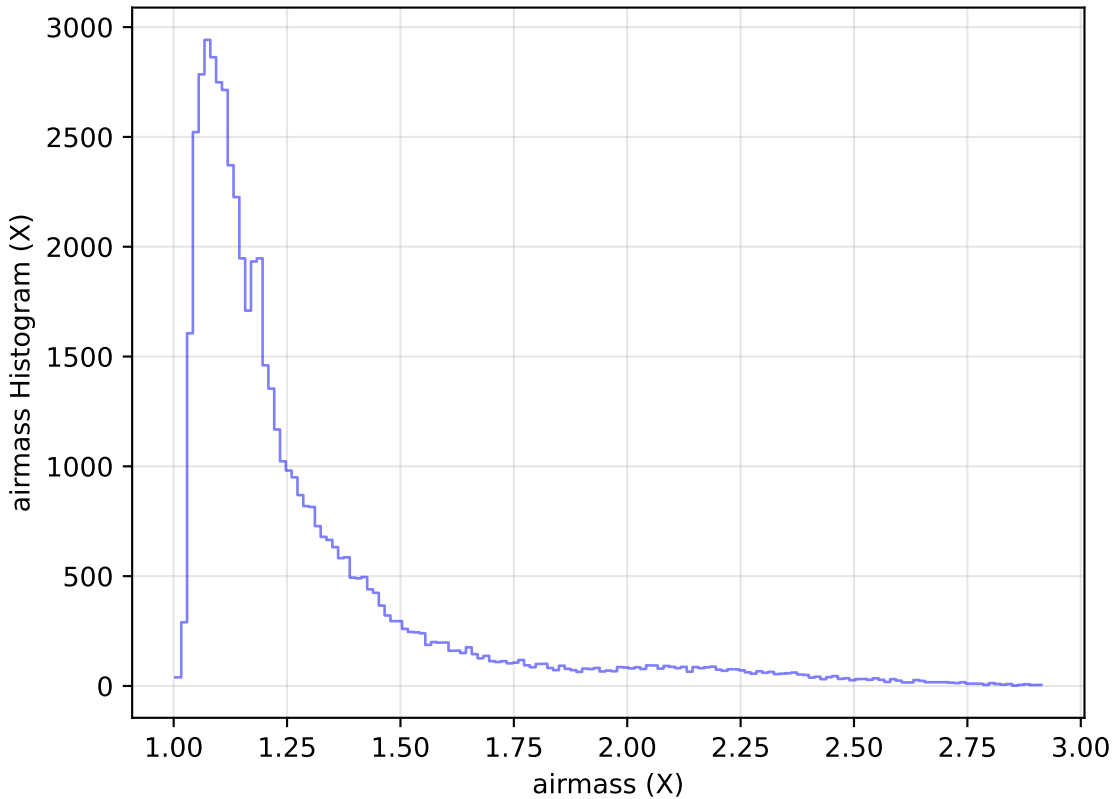
too_elab_r32_d2_griz_v3.4_10yrs Yr 1 i band: airmass Histogram
