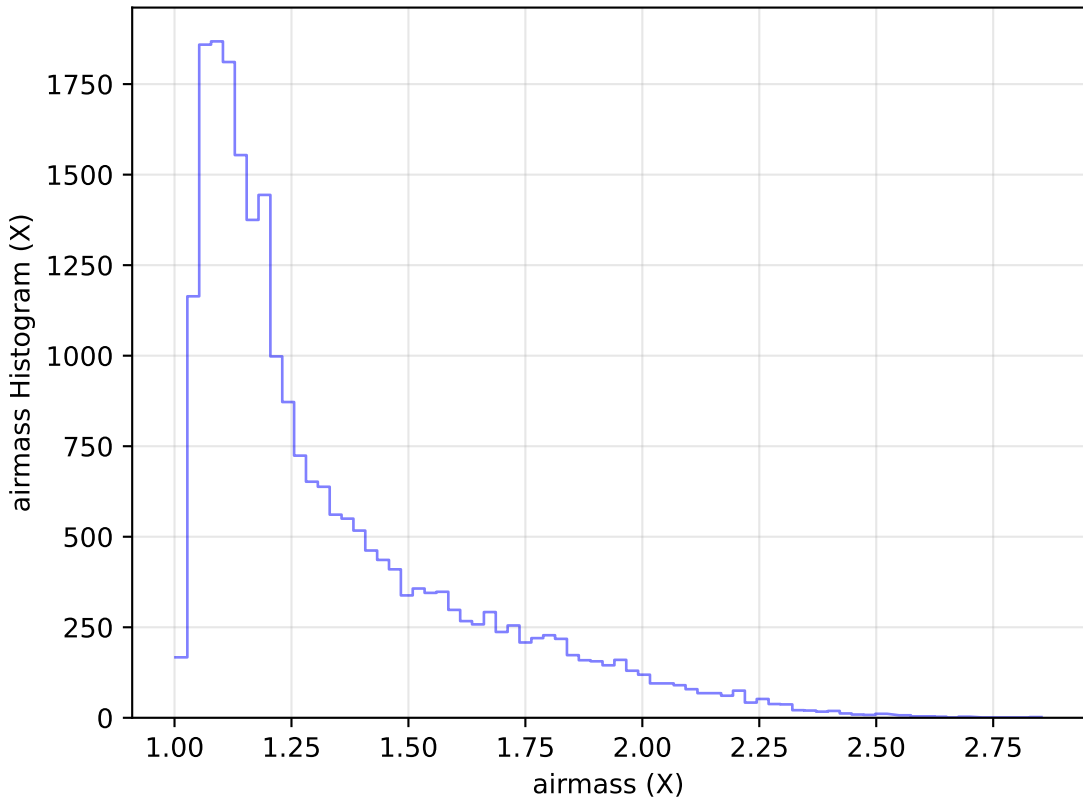
too_elab_r32_d2_griz_v3.4_10yrs Yr 1 g band: airmass Histogram
