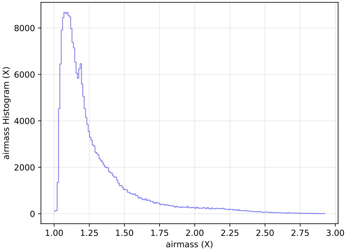
too_elab_r32_d2_griz_v3.4_10yrs Yr 1 all bands: airmass Histogram
