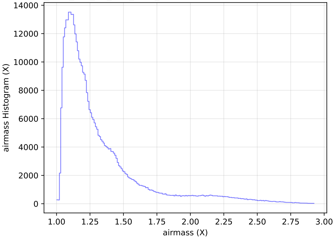
too_elab_r32_d2_griz_v3.4_10yrs WFD z band: airmass Histogram
