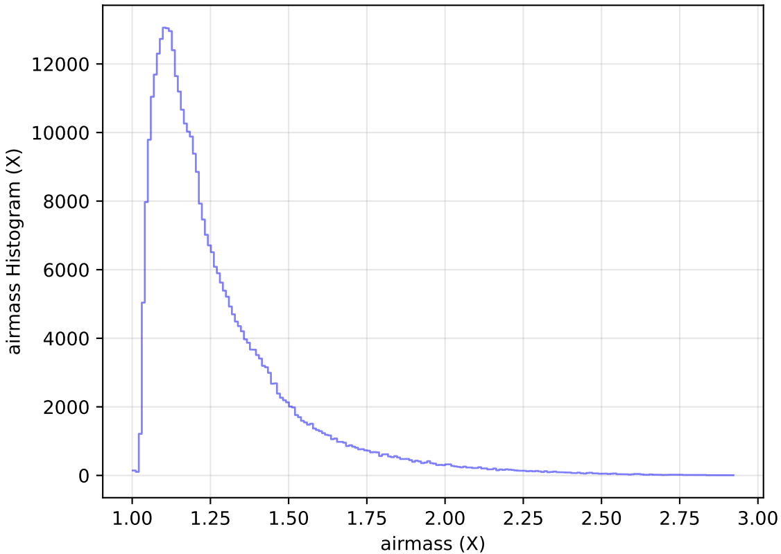
too_elab_r32_d2_griz_v3.4_10yrs WFD y band: airmass Histogram
