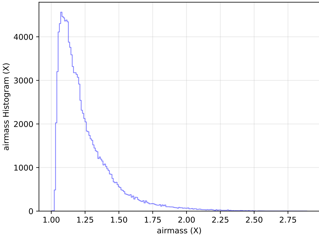
too_elab_r32_d2_griz_v3.4_10yrs WFD u band: airmass Histogram
