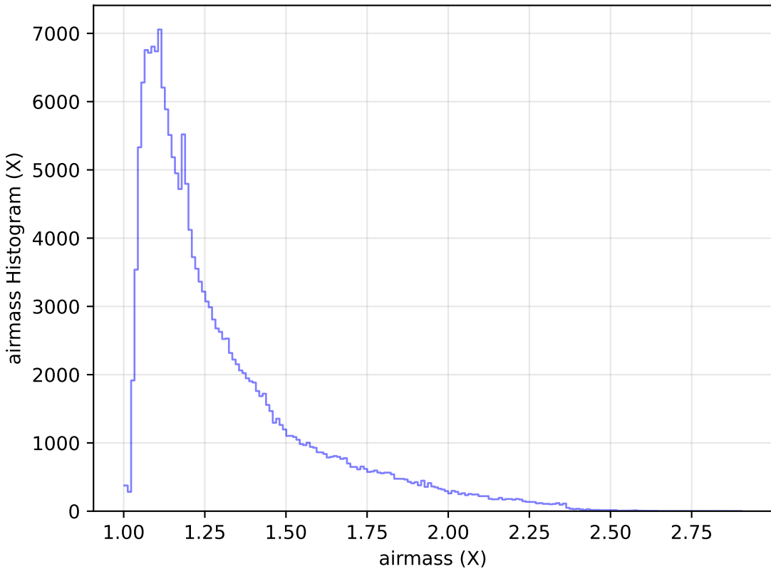
too_elab_r32_d2_griz_v3.4_10yrs WFD g band: airmass Histogram
