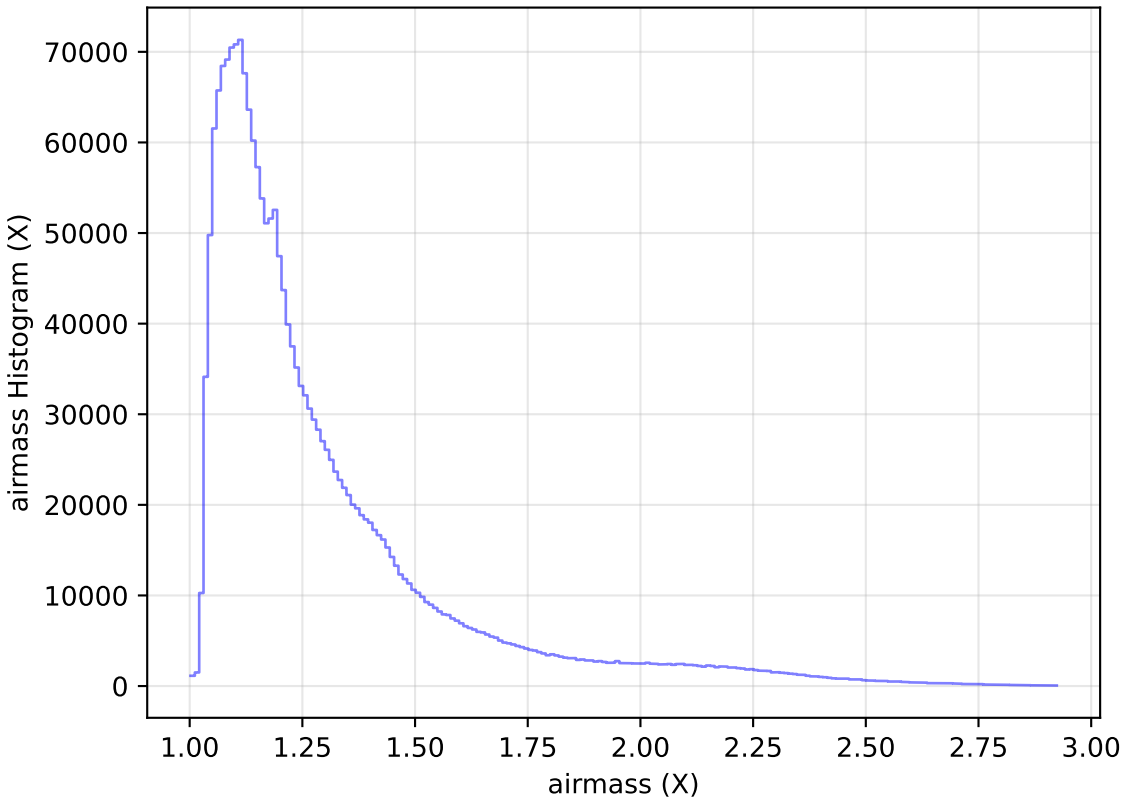
too_elab_r32_d2_griz_v3.4_10yrs WFD all bands: airmass Histogram
