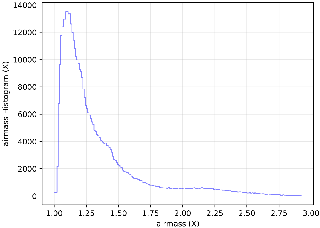
too_elab_r32_d2_griz_v3.4_10yrs All sky z band: airmass Histogram
