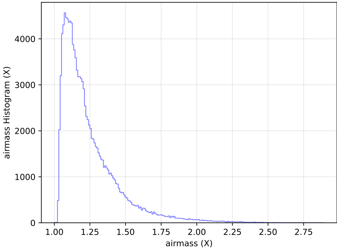
too_elab_r32_d2_griz_v3.4_10yrs All sky u band: airmass Histogram
