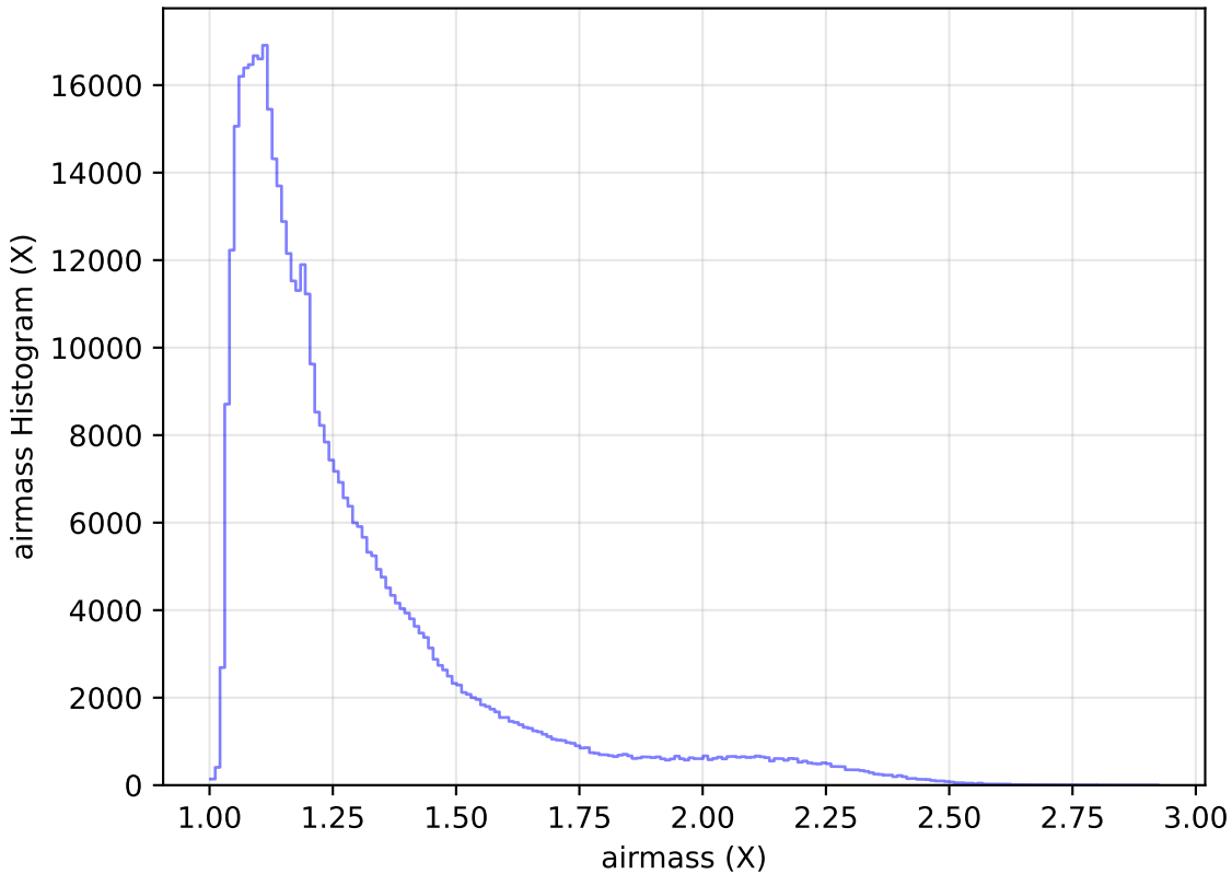
too_elab_r32_d2_griz_v3.4_10yrs All sky r band: airmass Histogram
