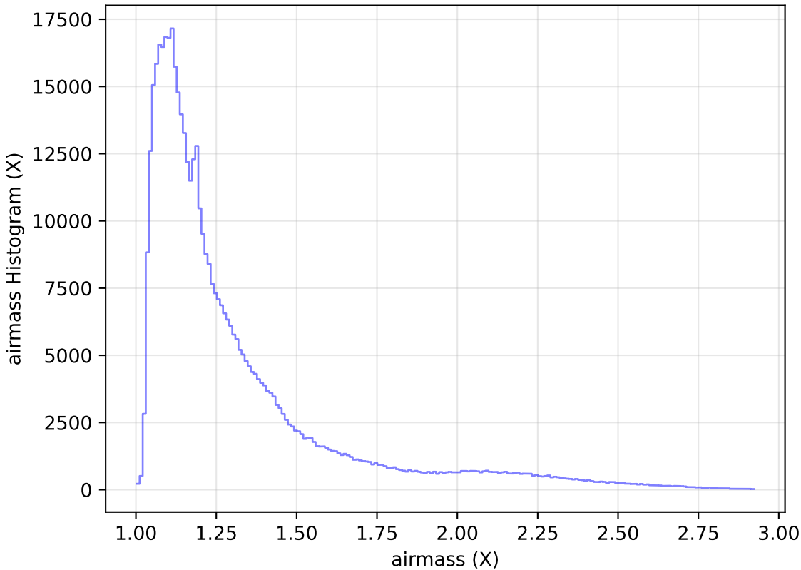
too_elab_r32_d2_griz_v3.4_10yrs All sky i band: airmass Histogram
