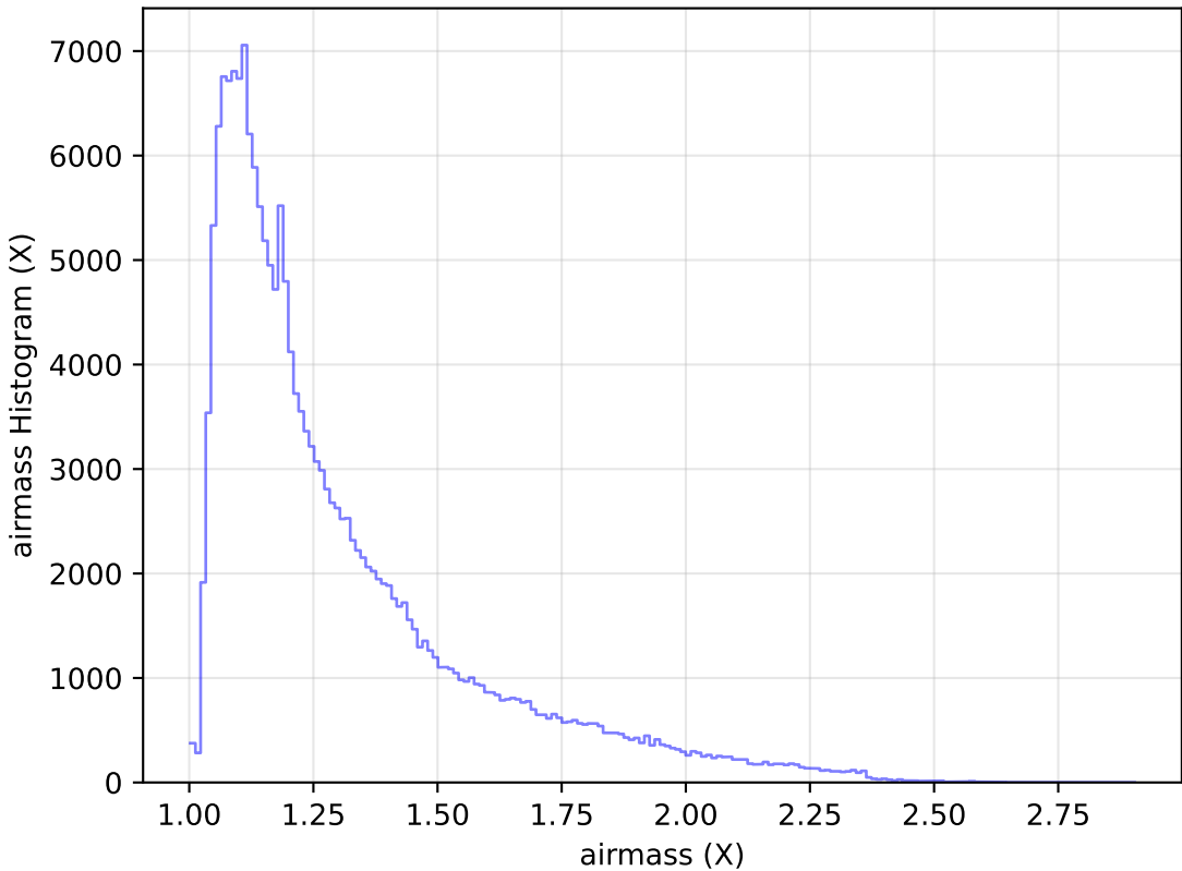
too_elab_r32_d2_griz_v3.4_10yrs All sky g band: airmass Histogram
