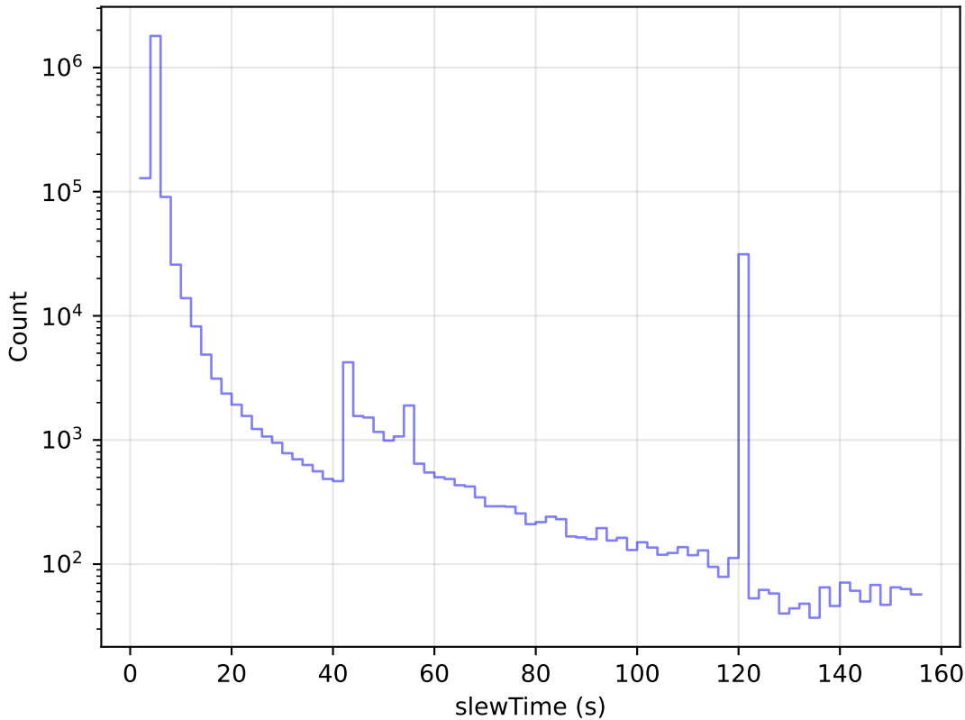
too_elab_r32_d2_griz_v3.4_10yrs All visits: Slew Time Histogram
