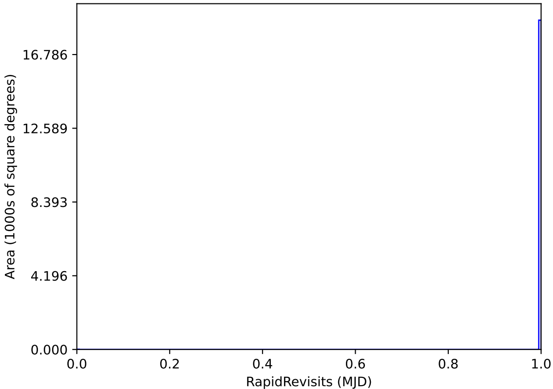
too_elab_r32_d2_griz_v3.4_10yrs WFD: RapidRevisits
