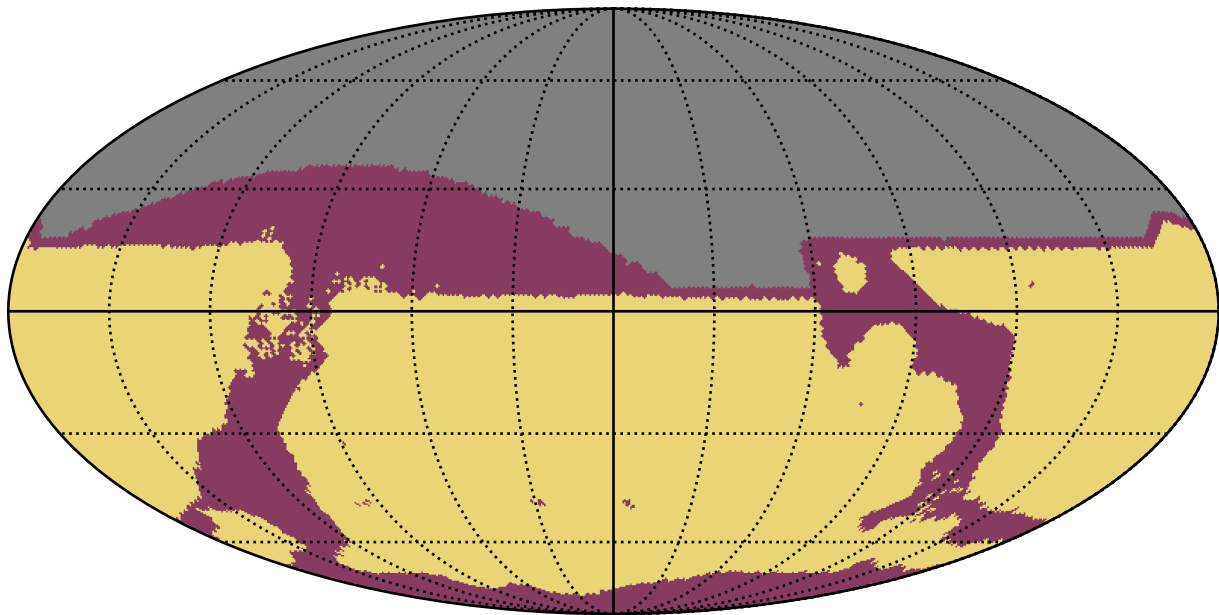
too_elab_r32_d2_griz_v3.4_10yrs All sky: RapidRevisits
