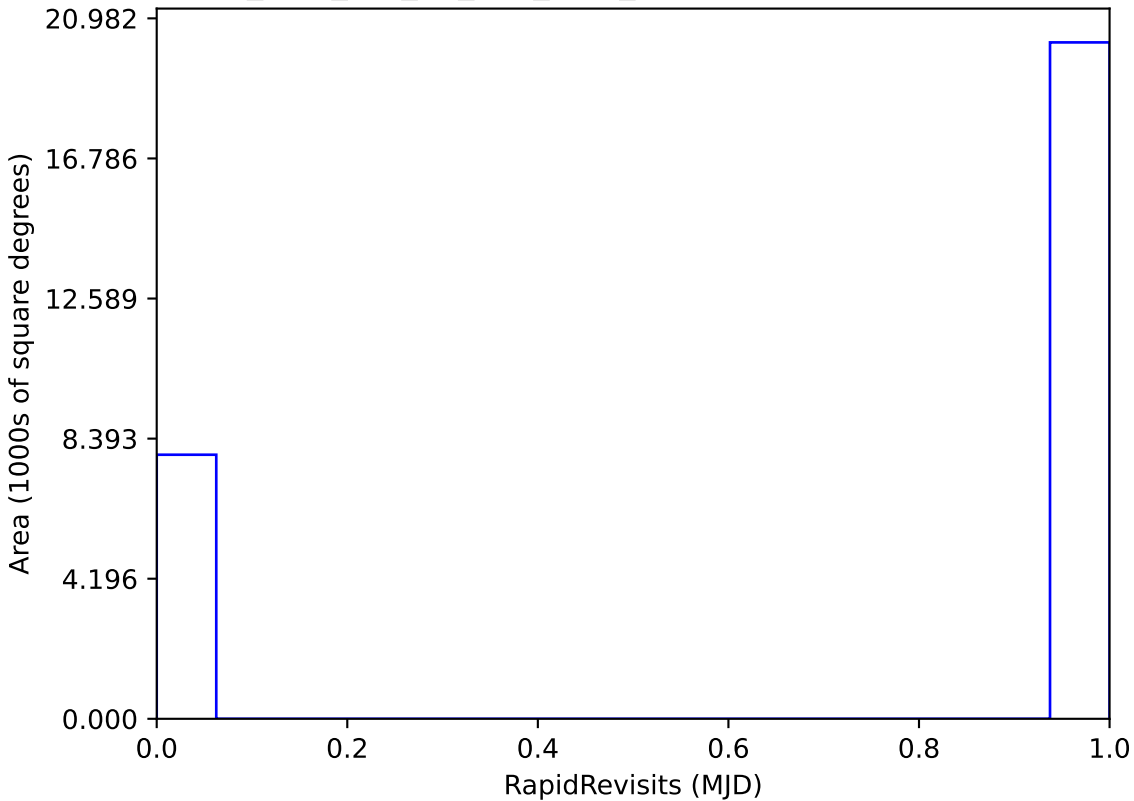
too_elab_r32_d2_griz_v3.4_10yrs All sky: RapidRevisits
