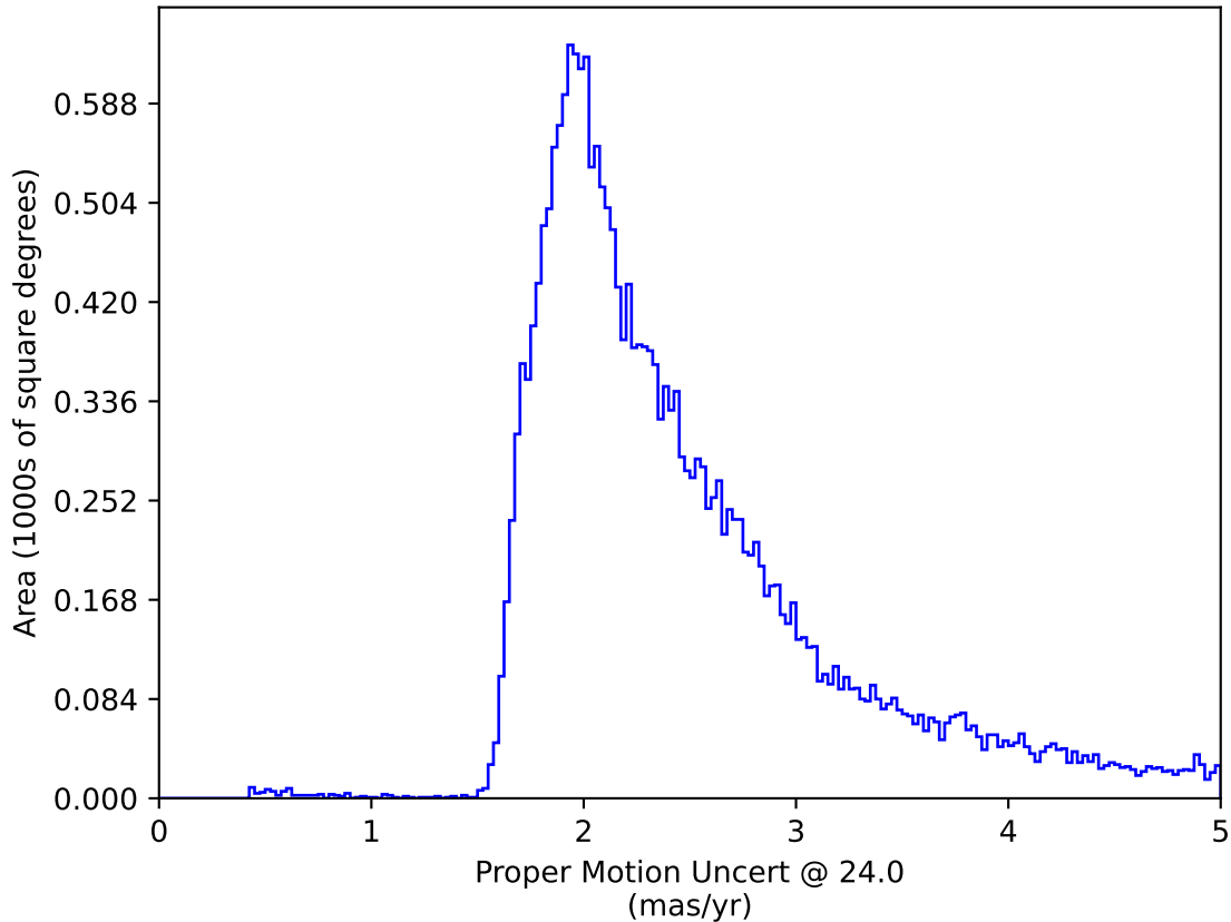
too_elab_r32_d2_griz_v3.4_10yrs All sky: Proper Motion Uncert @ 24.0
