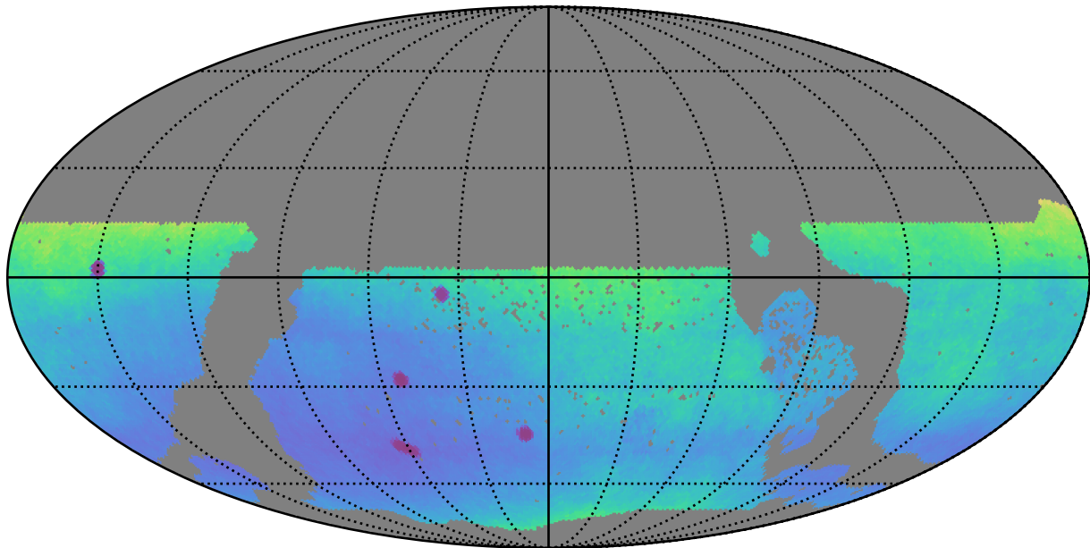
too_elab_r32_d2_griz_v3.4_10yrs WFD: Parallax Uncert @ 24.0
