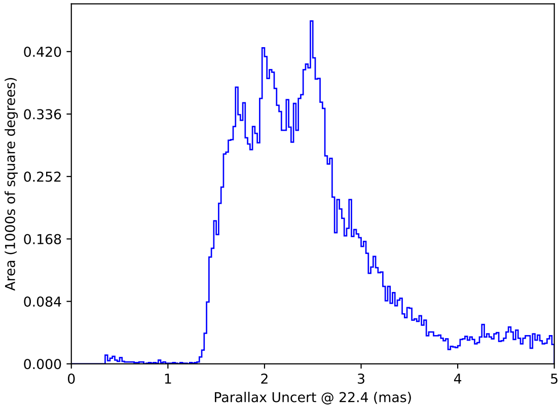
too_elab_r32_d2_griz_v3.4_10yrs All sky: Parallax Uncert @ 22.4
