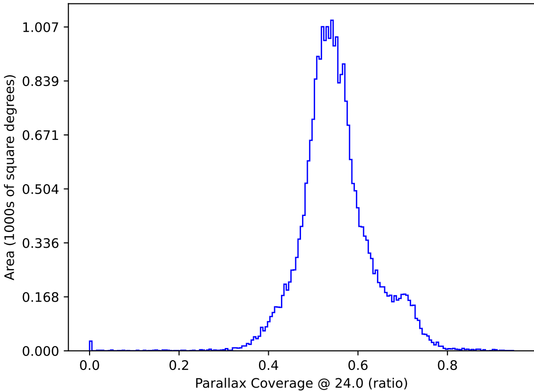
too_elab_r32_d2_griz_v3.4_10yrs All sky: Parallax Coverage @ 24.0
