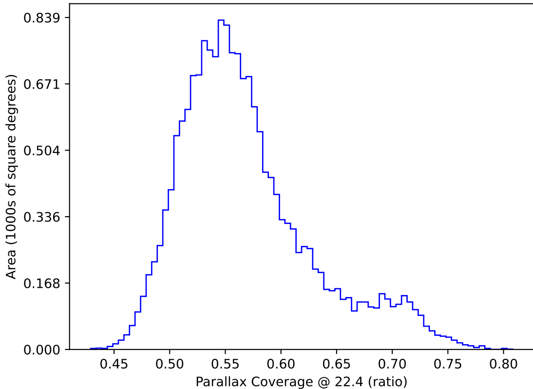
too_elab_r32_d2_griz_v3.4_10yrs WFD: Parallax Coverage @ 22.4
