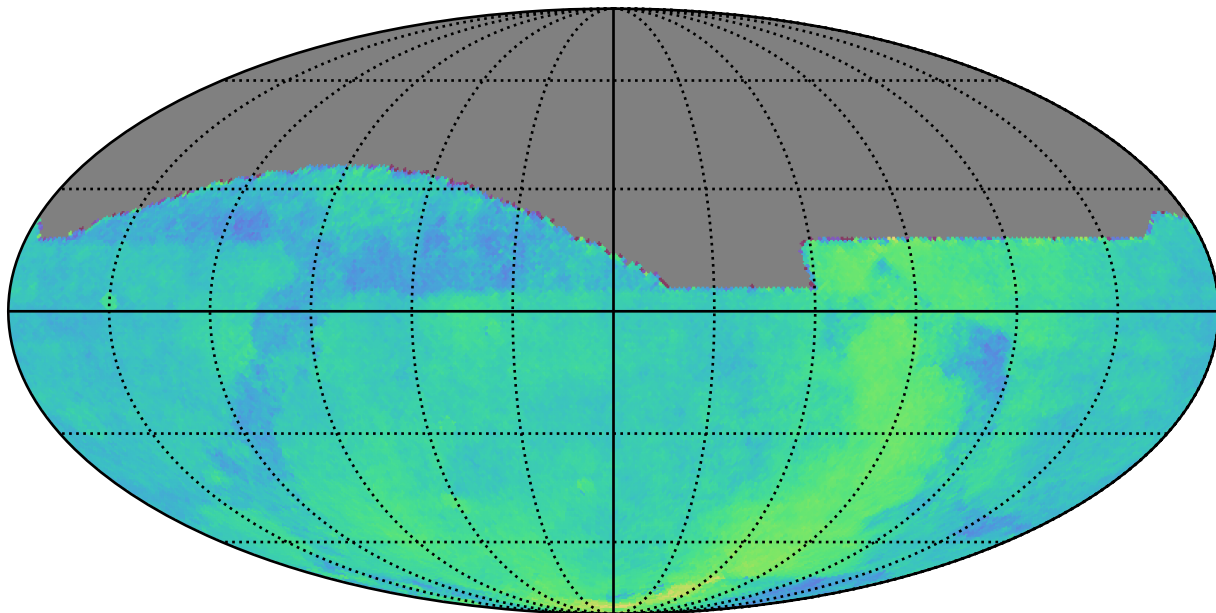
too_elab_r32_d2_griz_v3.4_10yrs All sky: Parallax Coverage @ 22.4
