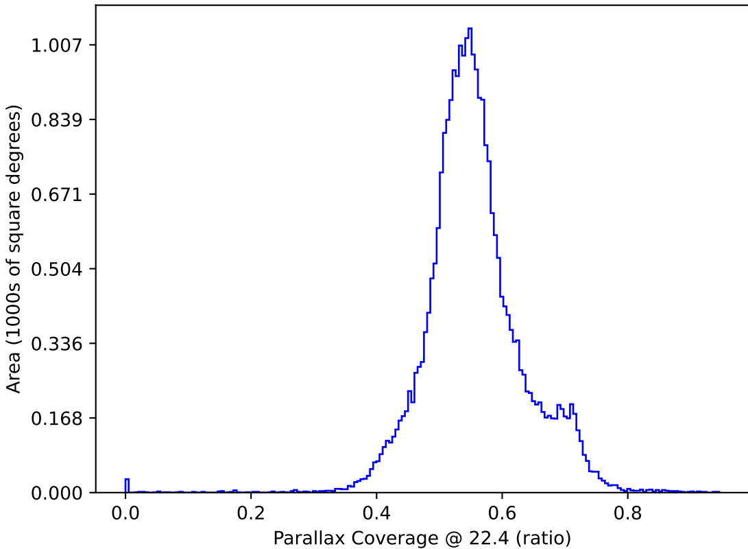
too_elab_r32_d2_griz_v3.4_10yrs All sky: Parallax Coverage @ 22.4
