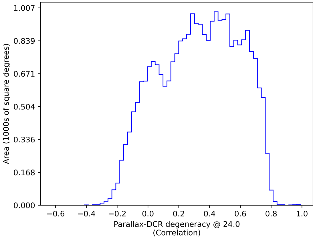
too_elab_r32_d2_griz_v3.4_10yrs All sky: Parallax-DCR degeneracy @ 24.0
