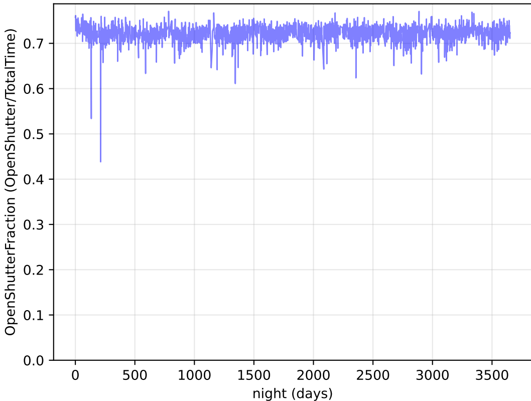
too_elab_r32_d2_griz_v3.4_10yrs Per night: OpenShutterFraction
