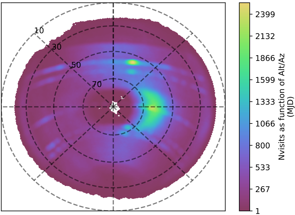
too_elab_r32_d2_griz_v3.4_10yrs z band: Nvisits as function of Alt/Az
