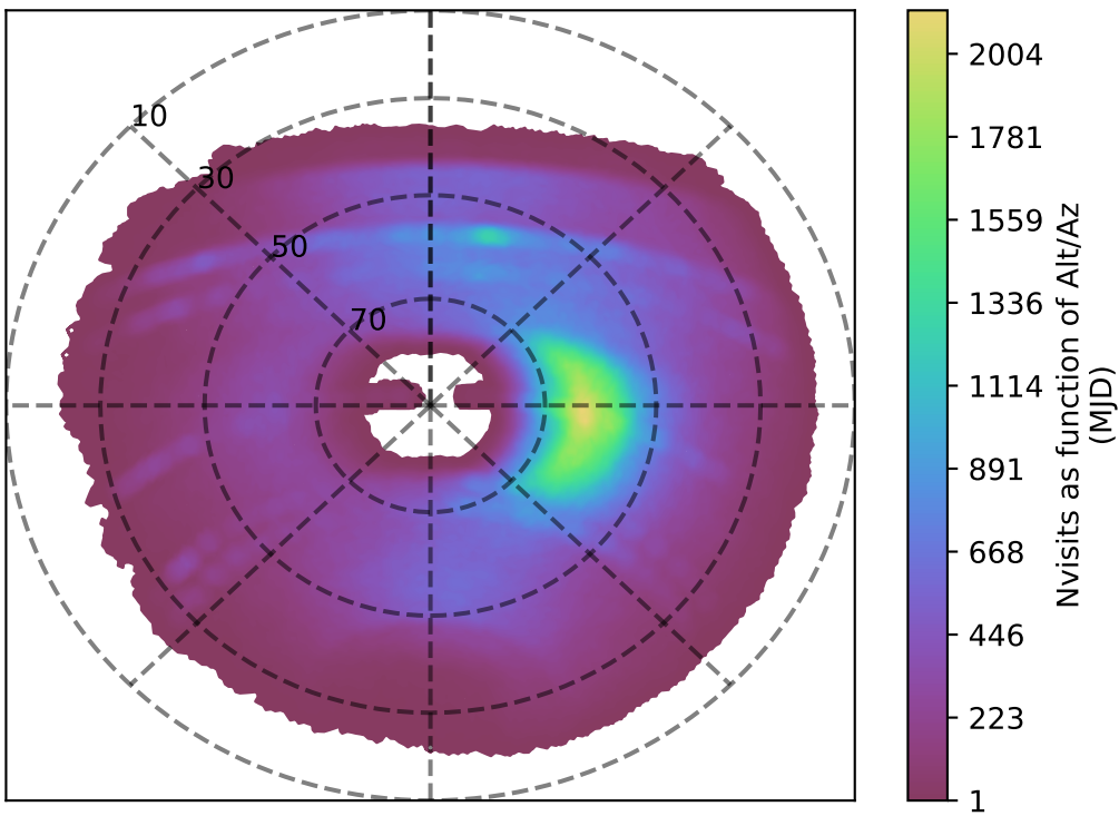
too_elab_r32_d2_griz_v3.4_10yrs y band: Nvisits as function of Alt/Az
