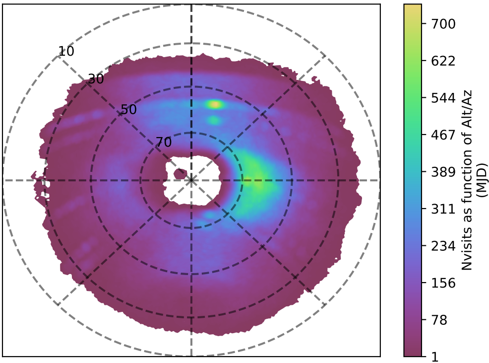
too_elab_r32_d2_griz_v3.4_10yrs u band: Nvisits as function of Alt/Az
