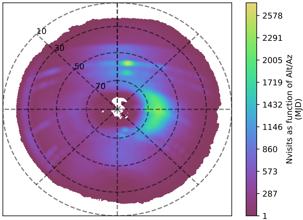
too_elab_r32_d2_griz_v3.4_10yrs r band: Nvisits as function of Alt/Az
