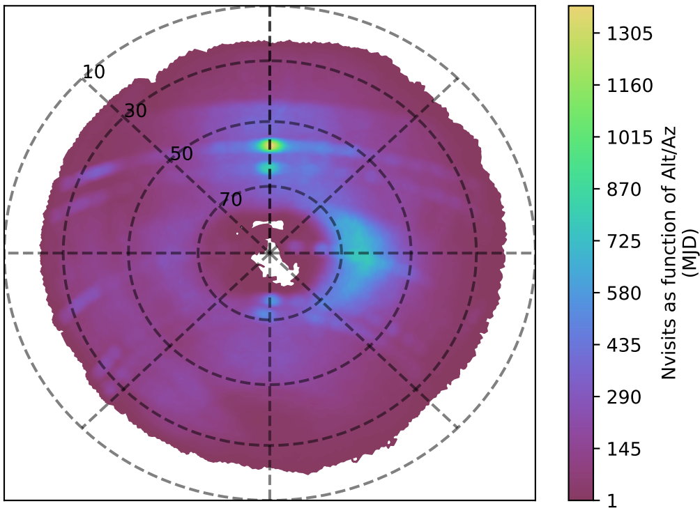
too_elab_r32_d2_griz_v3.4_10yrs g band: Nvisits as function of Alt/Az
