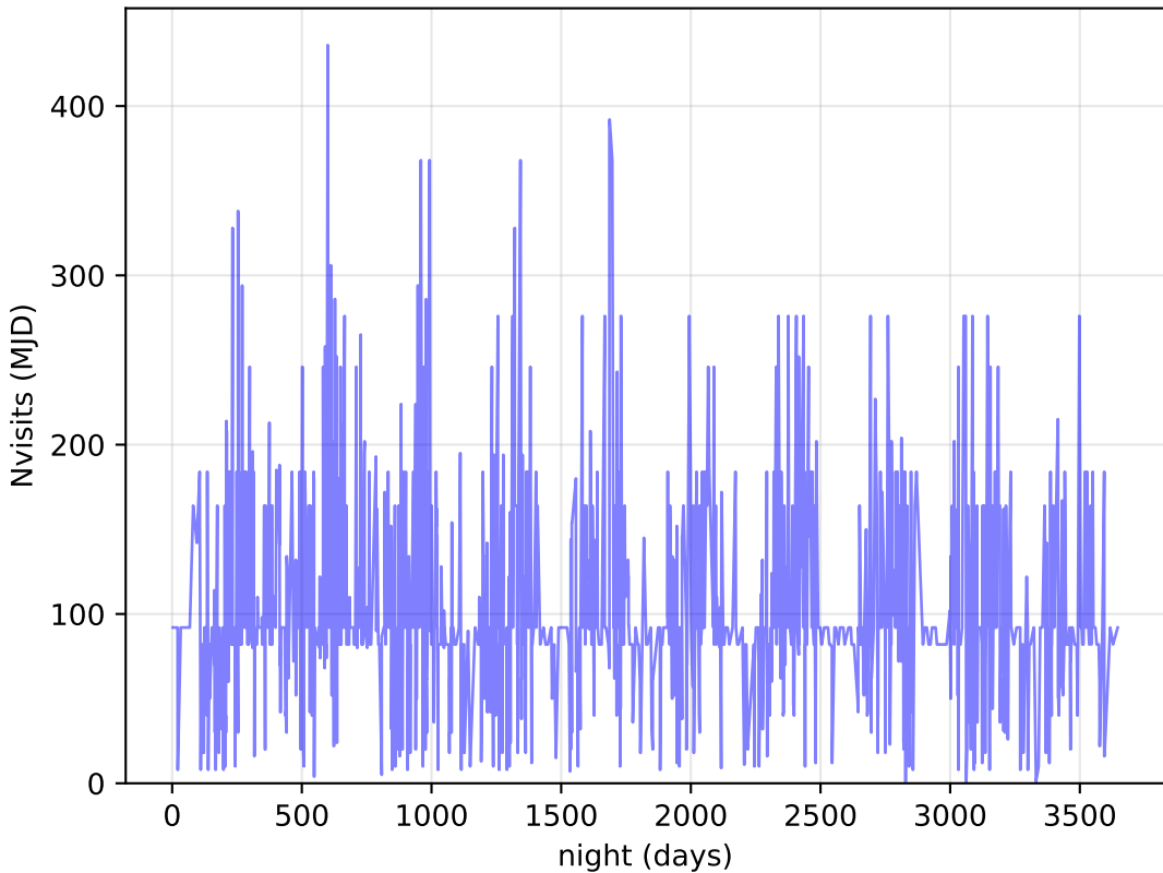
too_elab_r32_d2_griz_v3.4_10yrs DDF: Nvisits
