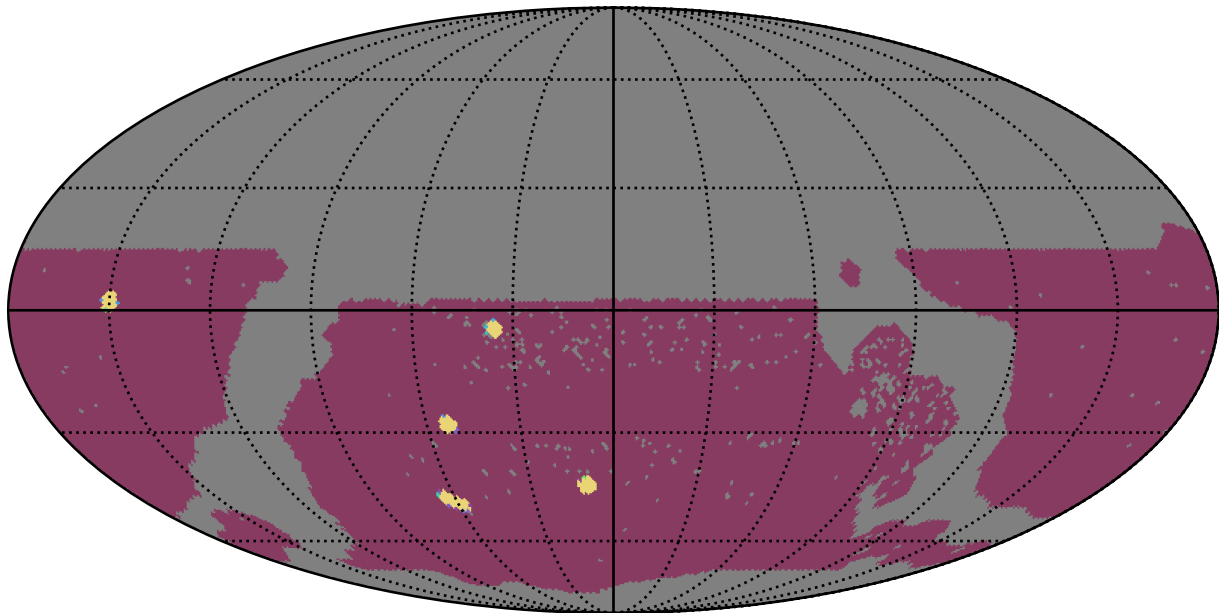
too_elab_r32_d2_griz_v3.4_10yrs WFD: NumberOfQuickRevisits
