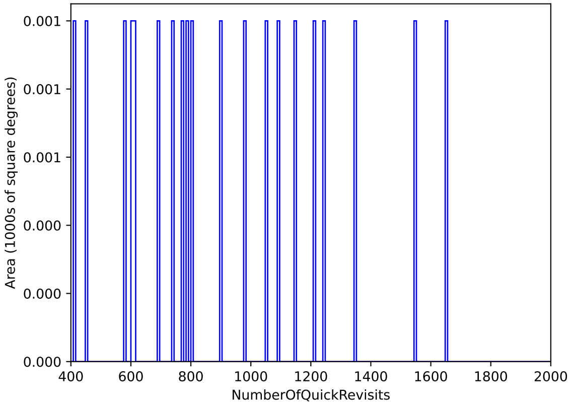
too_elab_r32_d2_griz_v3.4_10yrs WFD: NumberOfQuickRevisits
