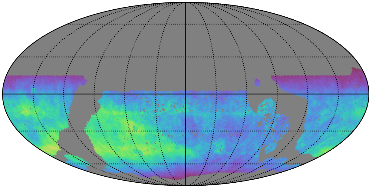
too_elab_r32_d2_griz_v3.4_10yrs WFD z band: Normalized Teff
