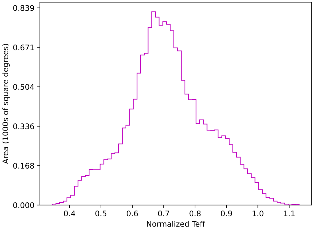
too_elab_r32_d2_griz_v3.4_10yrs WFD z band: Normalized Teff
